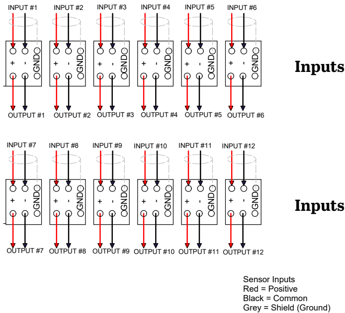
Figure 11. Field Wiring for Continuous Output
